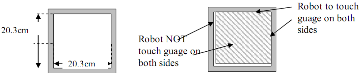
Figure 2: Caging Gauge
